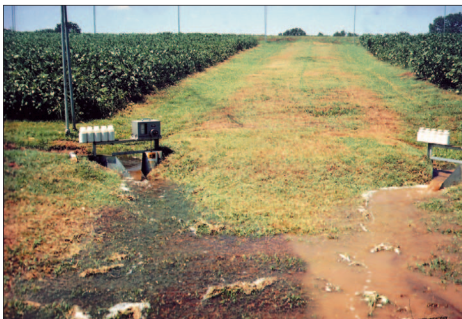
FIGURE 8. Runoff from no-till field on the left and conventional tilled field on the right from plots at Milan Experimental Station, Milan, Tennessee. The clear water from the no-till side of the field is transporting significantly less topsoil, nutrients, and pesticides.
